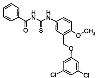
Compound # 46
